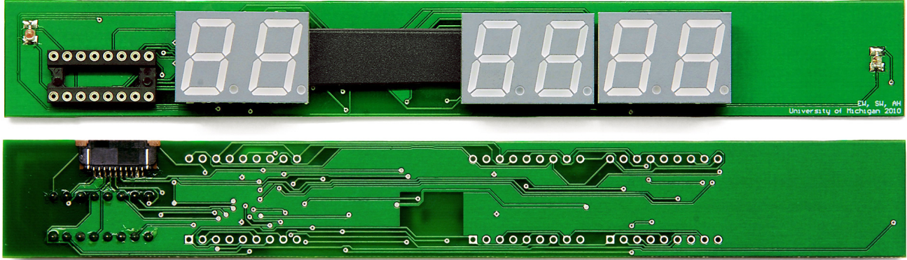
Figure 5: Dishonest Display Attack — We developed a dishonest display board, shown here at actual size. It looks almost identical to the real display board inside the control unit, but it shows fraudulent vote totals when results are counted. The only visible component on the reverse side is a programming connector, which could be removed before deploying the attack. Malicious election insiders or other criminals could install dishonest displays with little outward evidence of tampering.
