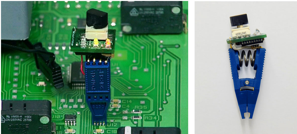
Figure 7: Clip-on Memory Manipulator Attack — We developed an attack device that can interface with the EVM’s memory to change votes or violate ballot secrecy. It attaches directly to the memory chips that store the votes in the control unit ( left ). Shown actual size ( right ), the device fits in a shirt pocket.
