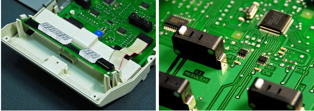
Figure 4: The display board in the control unit ( left ) is a simple electric circuit containing only LEDs and a connector. Note that the 7-segment LEDs are raised slightly by a black plastic spacer. Most of the machine’s logic is contained on the control unit main board , including the processor ( right, rear ) and two EEPROM memory chips that store the vote data ( right, center ).
